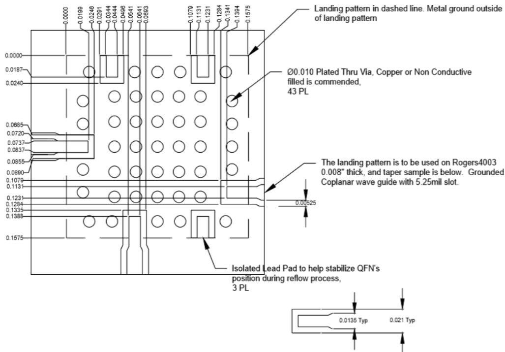
QFN-Package Surface-Mount Landing Pattern
